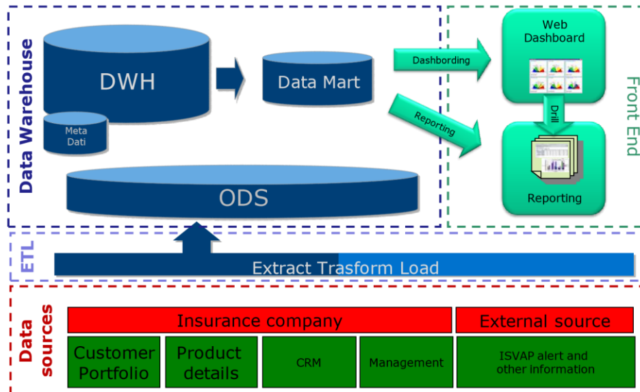
Figure 3. Applicative architecture of system GIACO LS.
